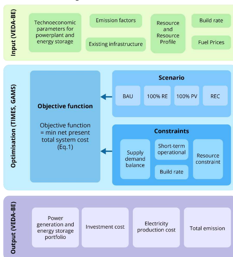
Figure 17. Model Framework
