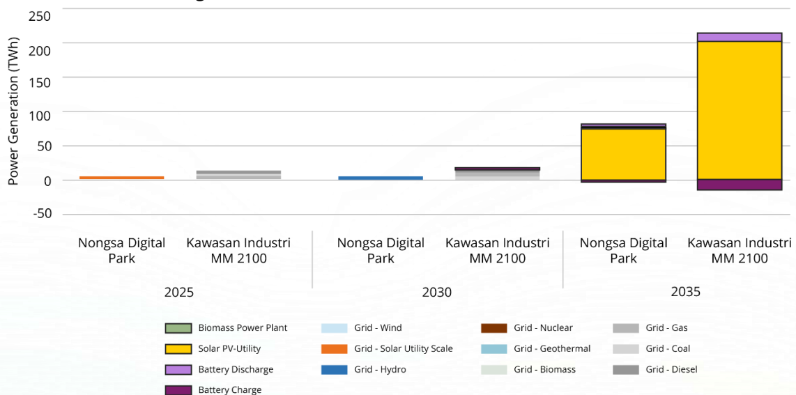
Figure 23. Power Generation Mix for 100% PV Scenario
